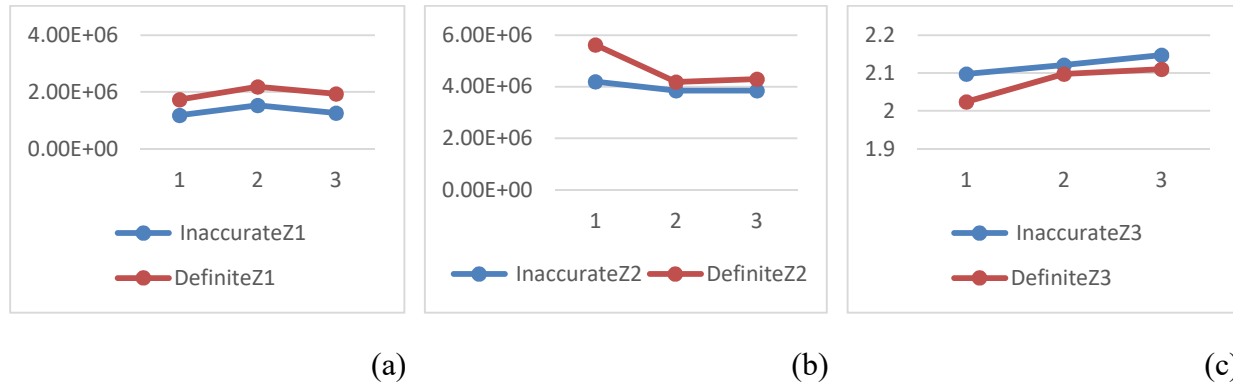
Figure 8. Comparison graphs of functions in two imprecise and definite cases: (a) Graph of the first objective function ( z_1 ), (b) Graph of the second objective function ( z_2 ), and (c) Graph of the third objective function ( z_3 ).
