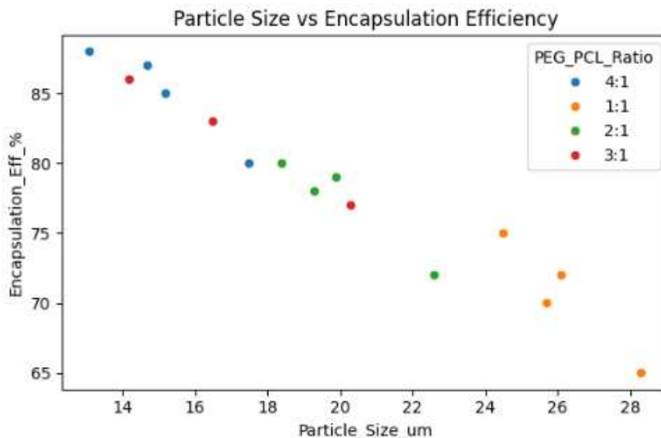
Figure 6. Interpretation of the Particle Size vs Encapsulation Efficiency Chart
