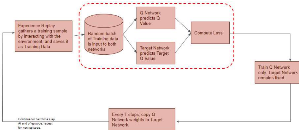
Fig 3.1: Deep Q-Networks
